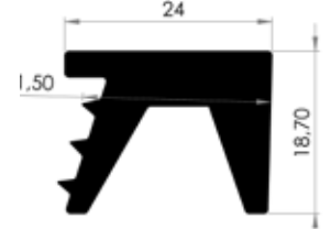
V TİP PANEL
